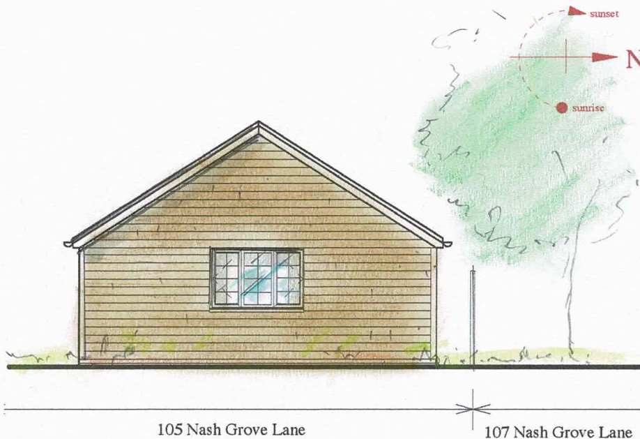
SIDE/EAST ELEVATION
